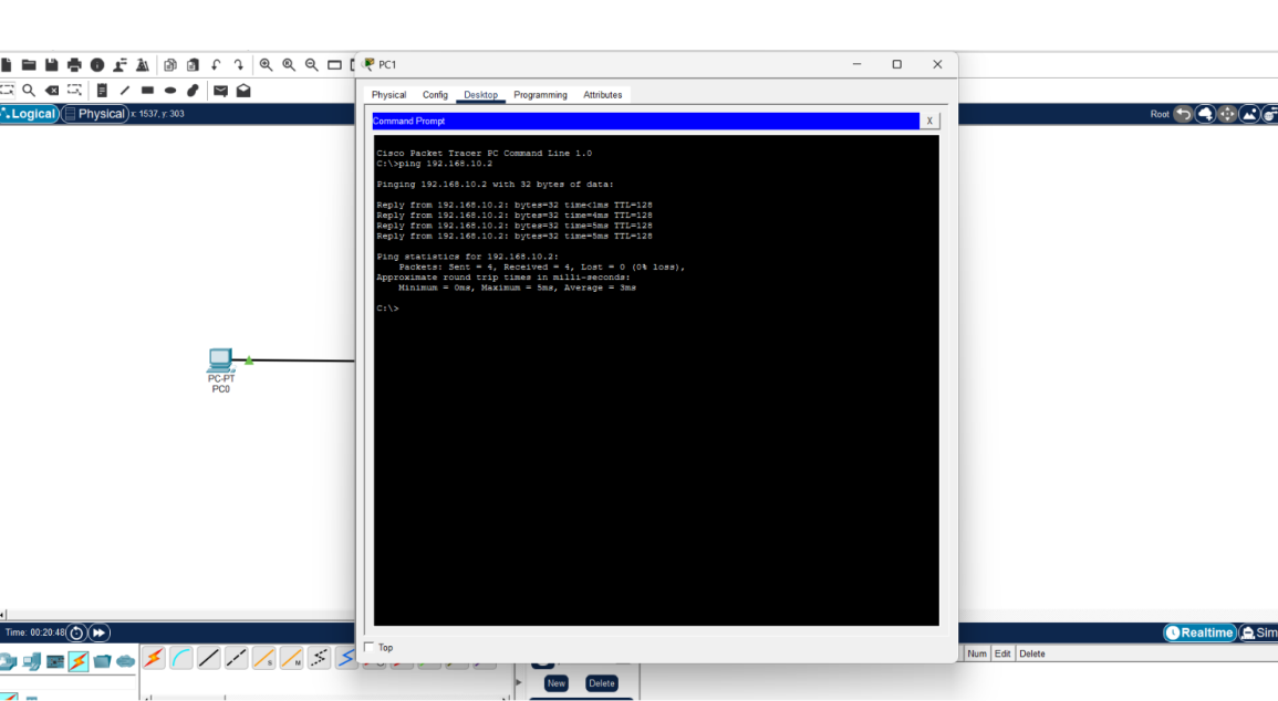
ScreenShot 2:
