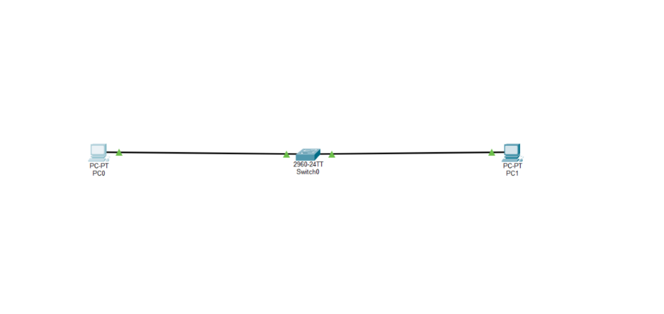
ScreenShot 2:
