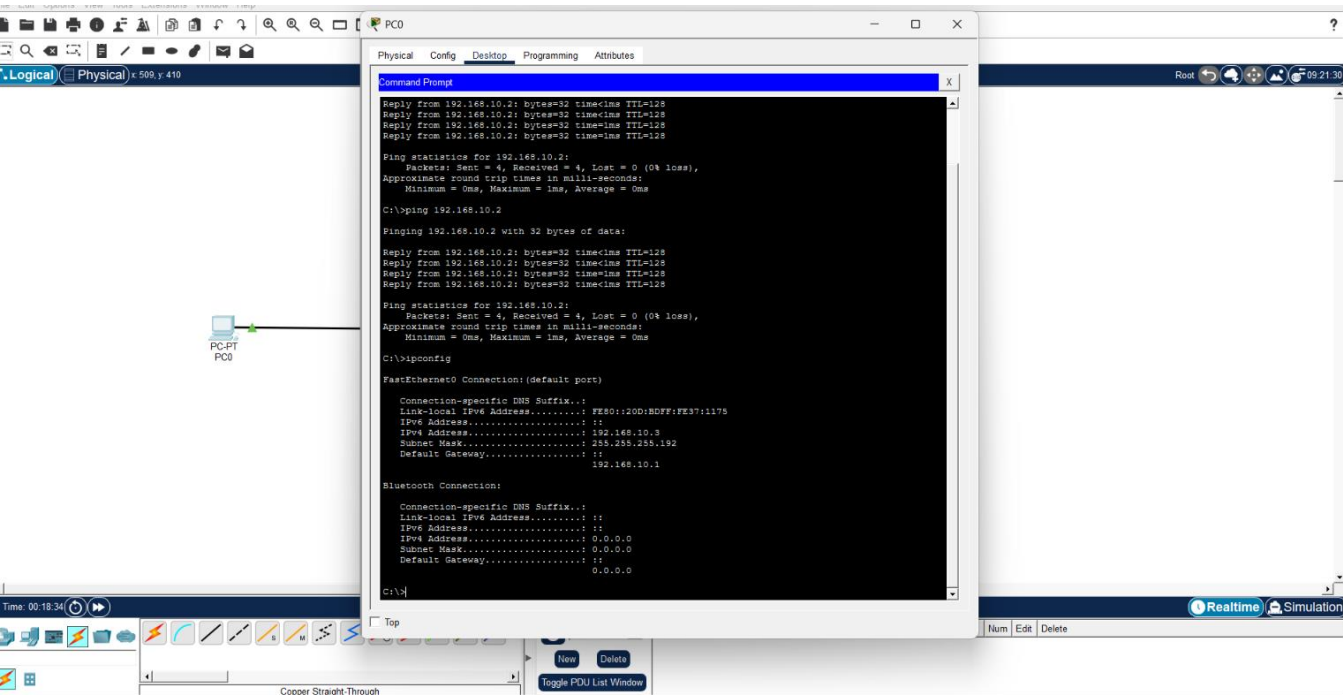
Screen shot 3:
